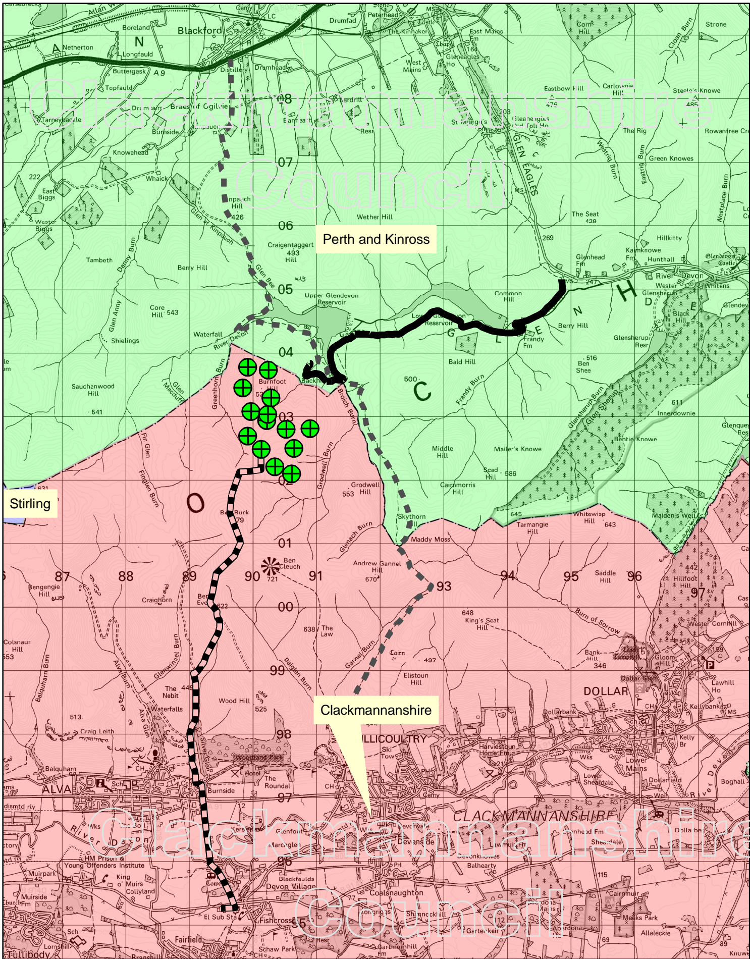
Plan 1: Location plan for the proposed wind-farm on Burnfoot Hill
